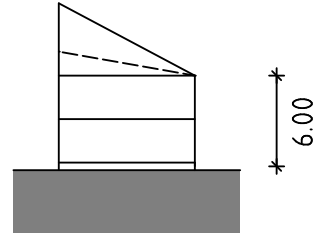
E+I Pultdach 10°-30°
